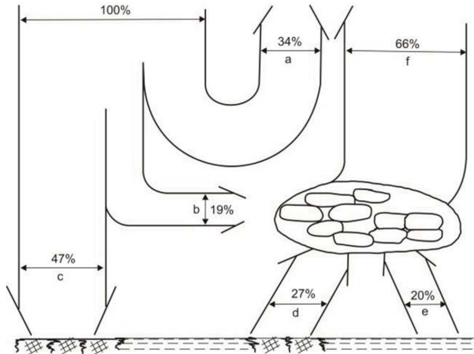
Figure 1. Balance of solar energy.
